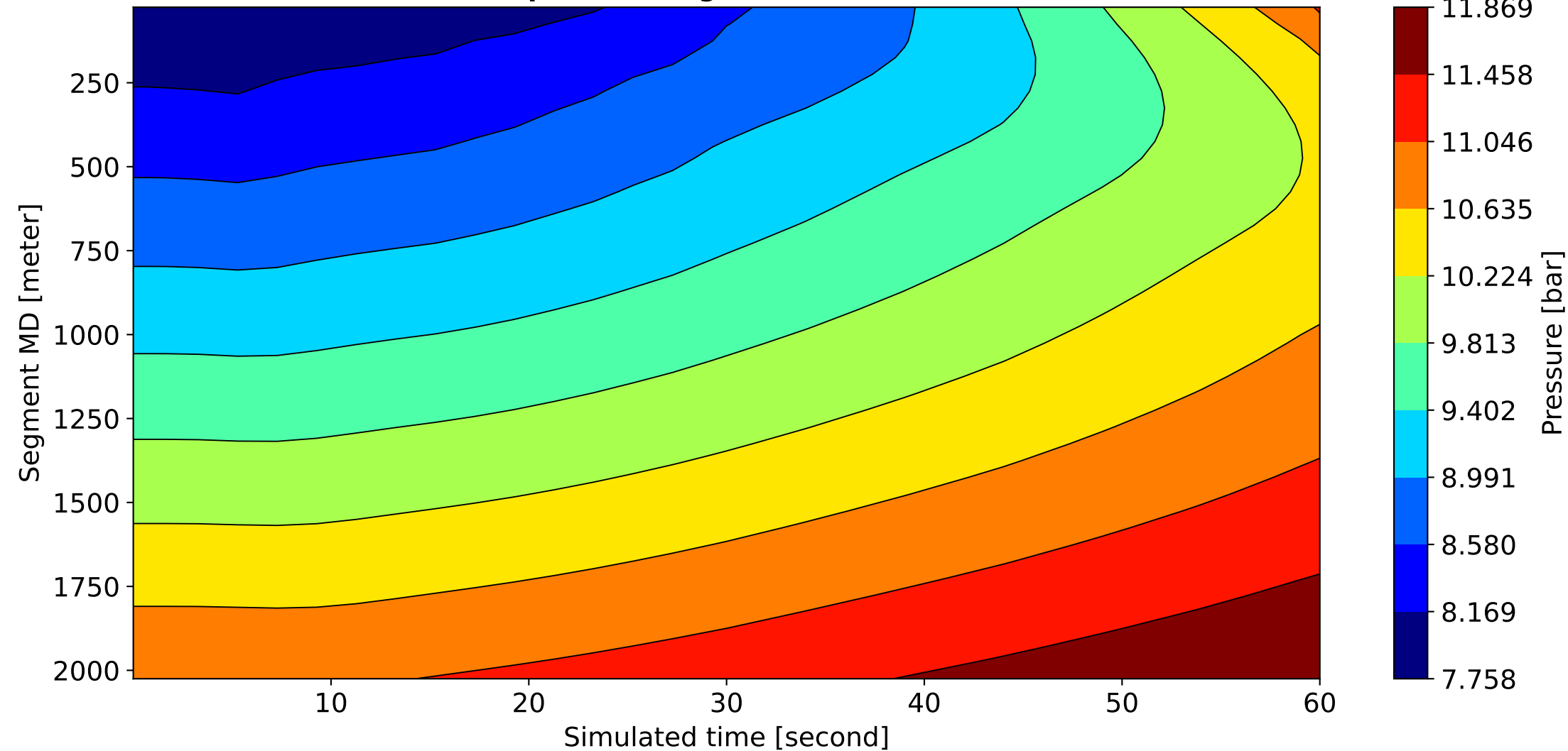
Pressure profile along the wellbore over time
